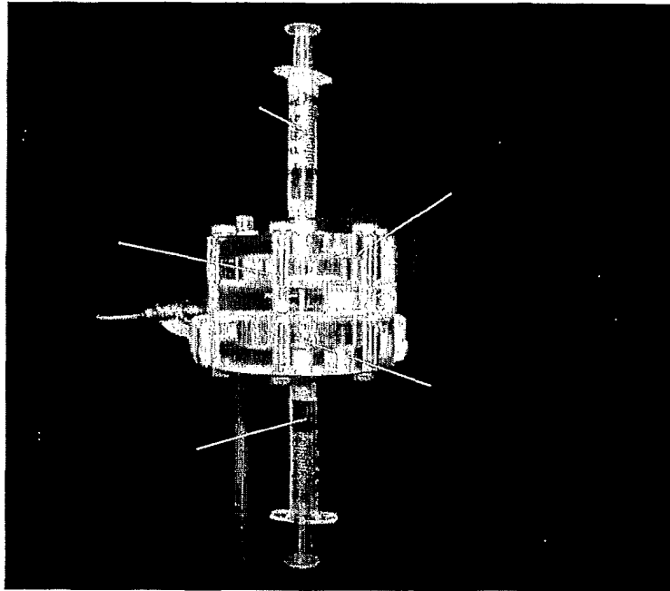
Fig. 17. Plexiglas, water-tight CTM macro-model for pressure analysis
